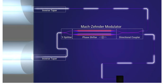
Fig. 1. Schematic representation of a Mach-Zehnder Interferometer (MZI) electro-optic modulator.
