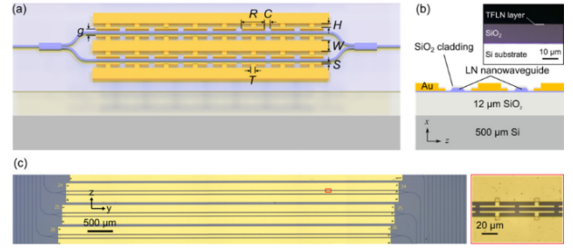
Fig. 4. (a) Schematic of the EOM. (b) Cross-section showing the thick silica buffer beneath the waveguide. (c) Top-down microscope image of the periodic T-rails.
