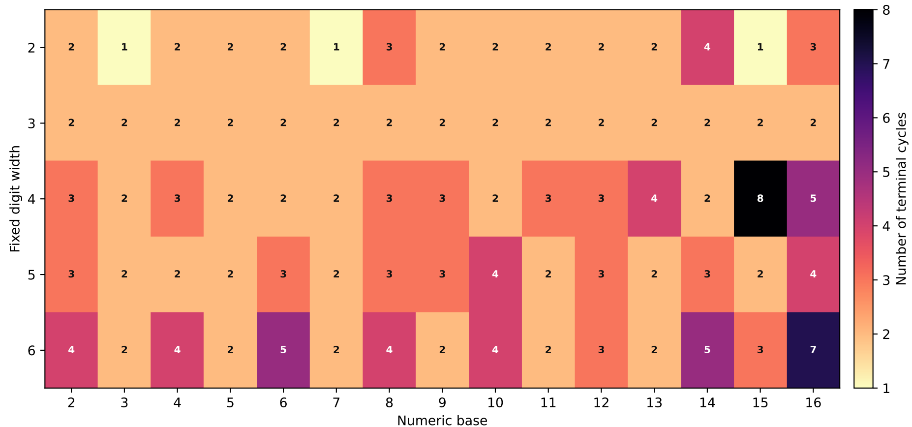
Kaprekar attractors across bases and digit widths
