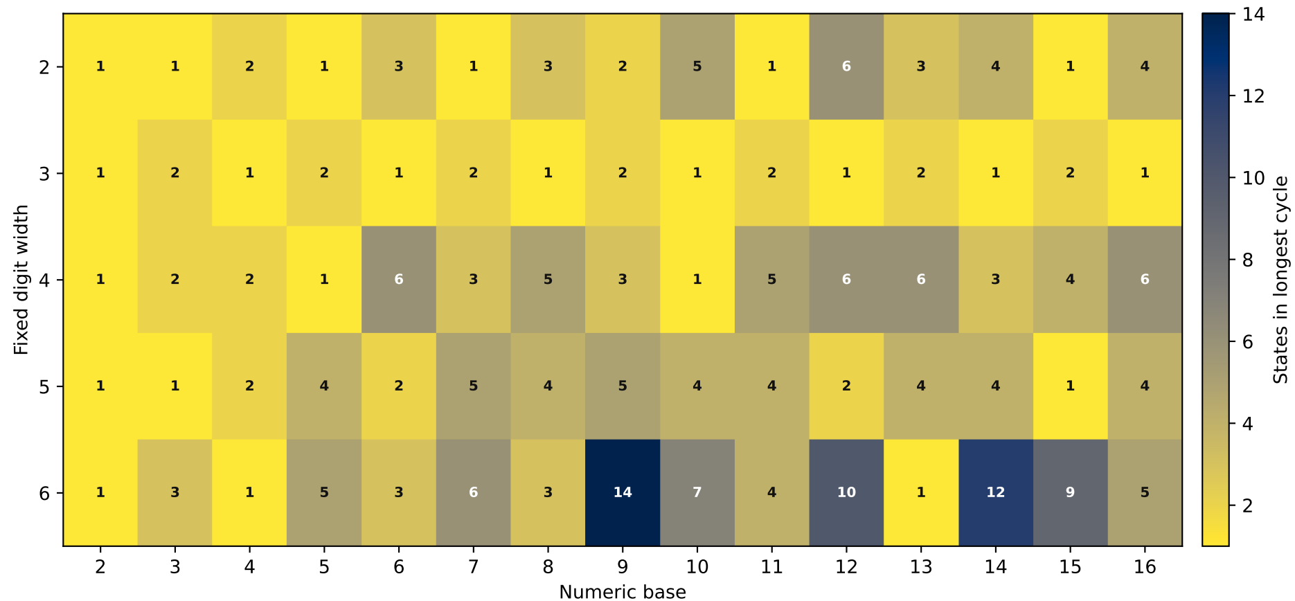
Maximum terminal cycle length
