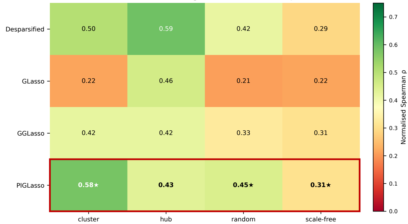
A Diffusion recovery — normalised Spearman \rho (mean across 3 configs \times 3 \delta -modes \times 50 reps)
