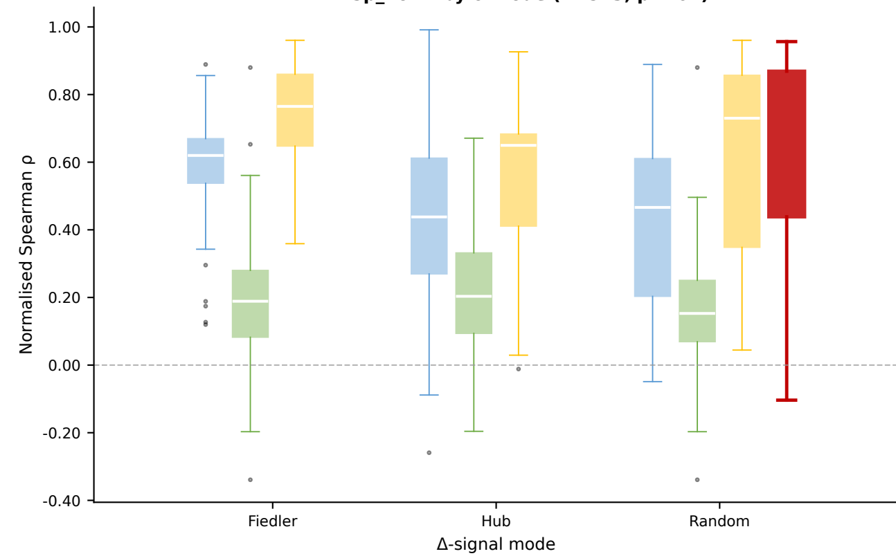
B DiffSp_norm by \delta -mode (n=513, p=164)
