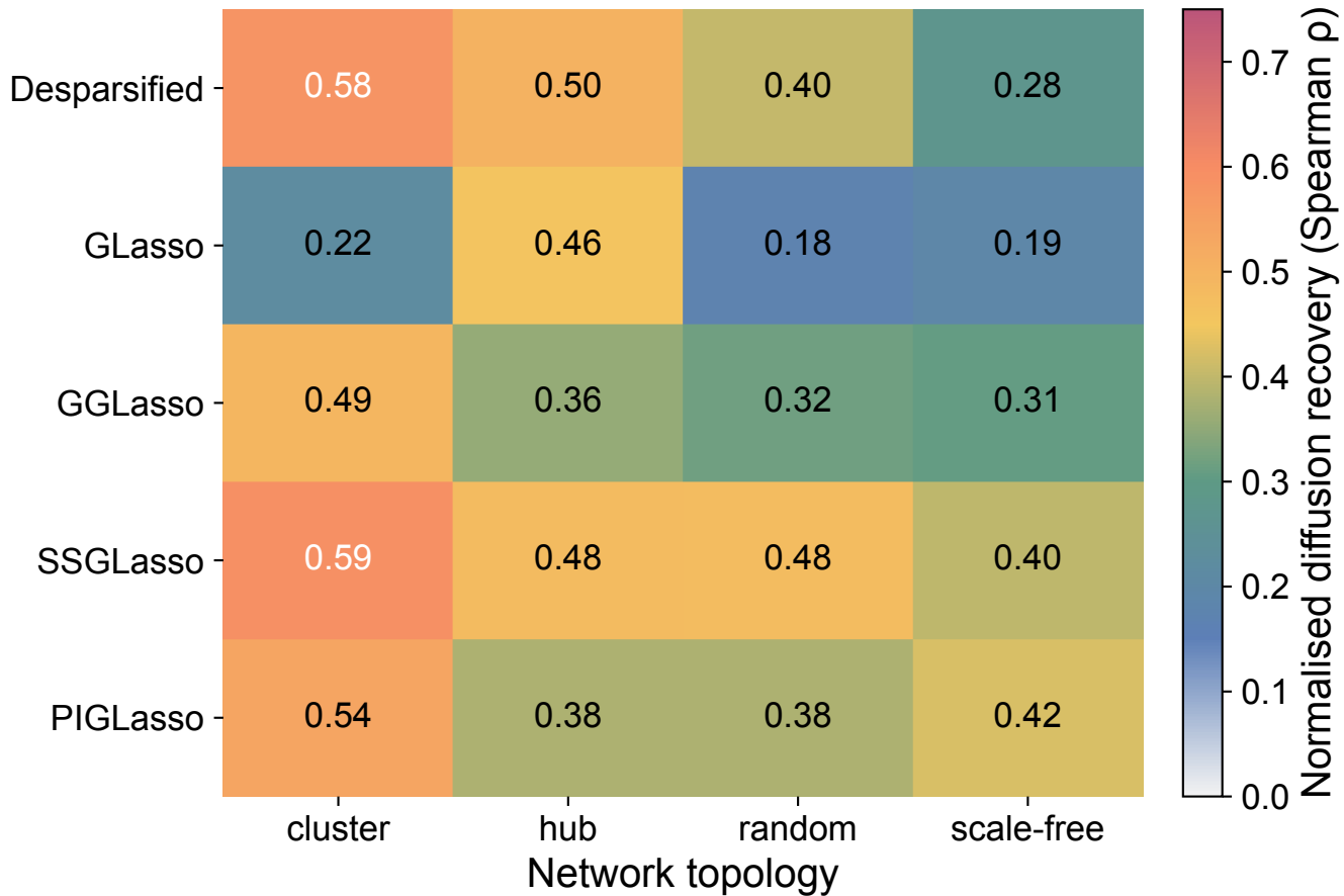
Inference method
