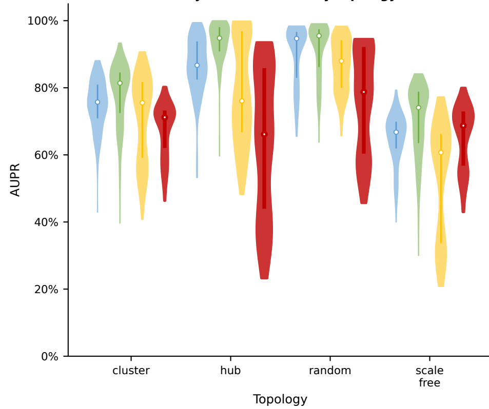
A Synthetic — AUPR by topology
