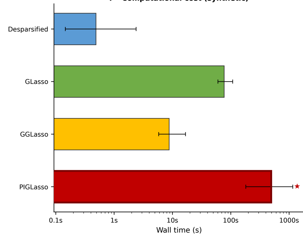
F Computational cost (synthetic)
