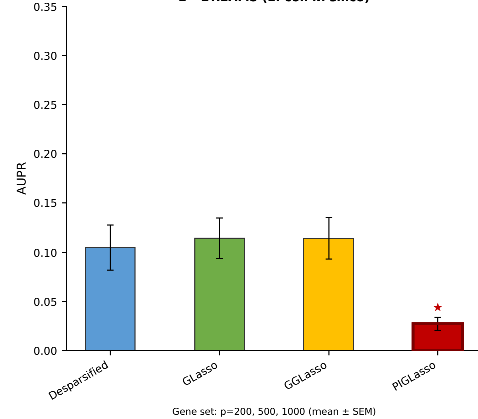
D DREAM5 (E. coli in silico)
