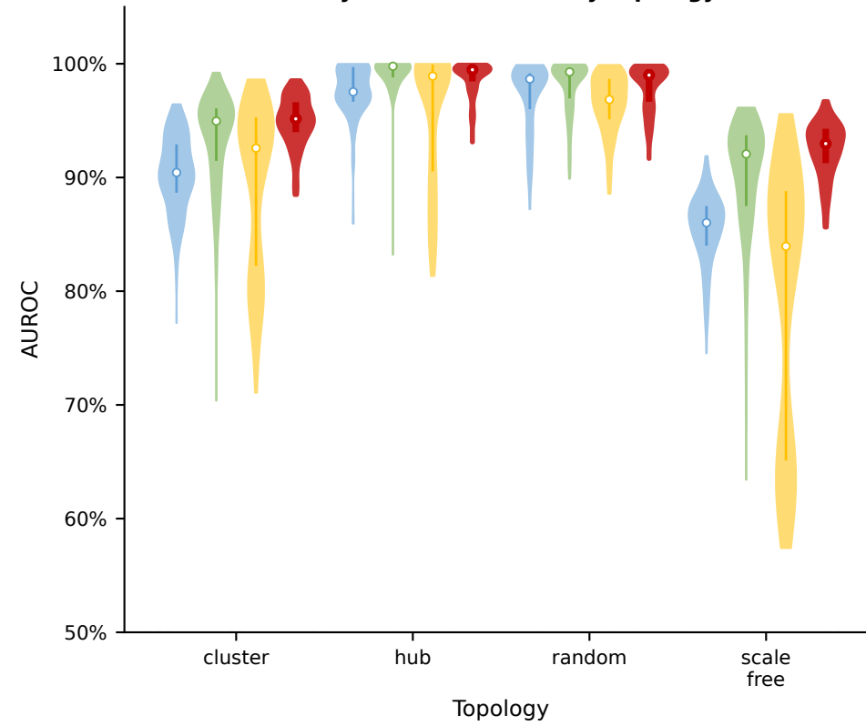
B Synthetic — AUROC by topology
