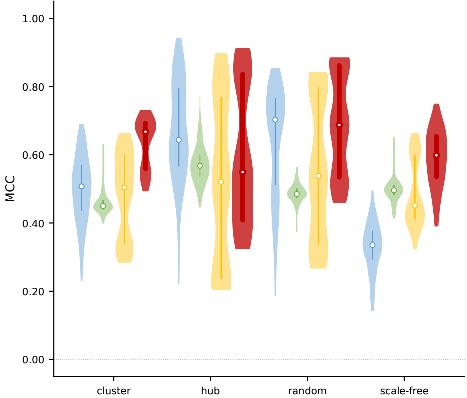
B Synthetic — MCC by topology
