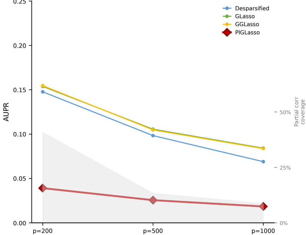
E DREAM5 — AUPR vs. gene-set size
