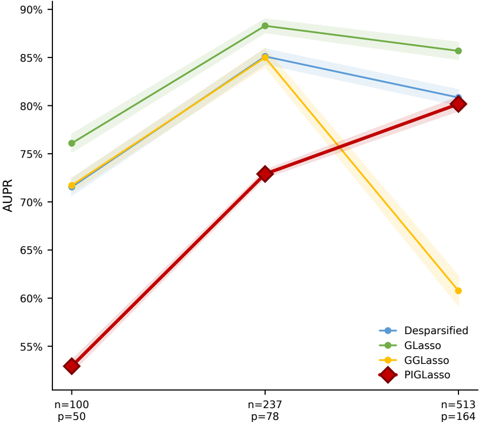
C Scalability — AUPR vs. problem size
