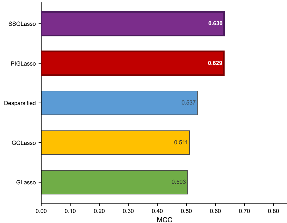
A Grand-mean MCC (synthetic, all topologies)
