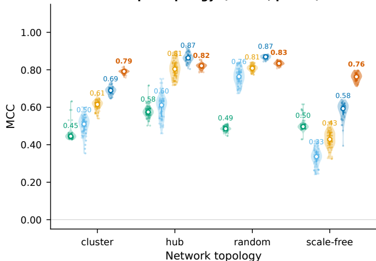
B MCC per topology (n=513, p=164)
