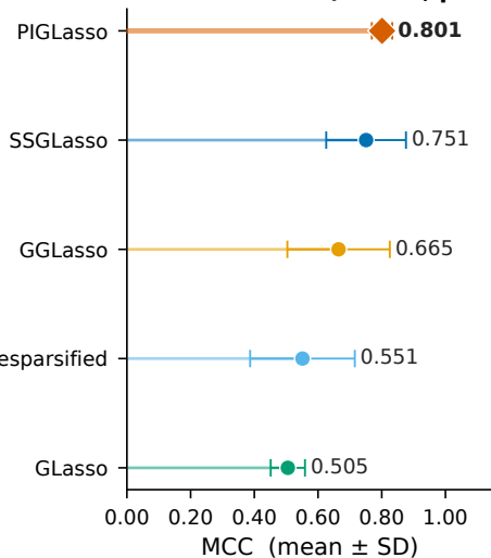
A Grand-mean MCC (n=513, p=164)
