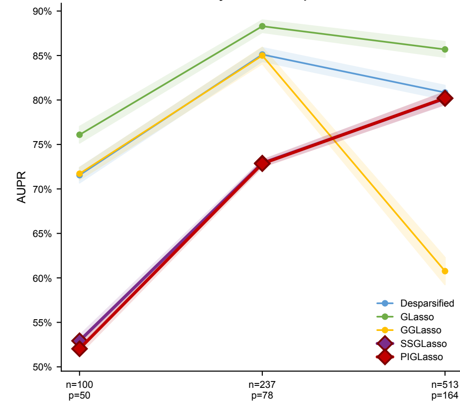
C Scalability — AUPR vs. problem size
