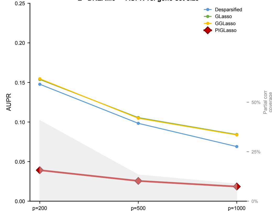
E DREAM5 — AUPR vs. gene-set size
