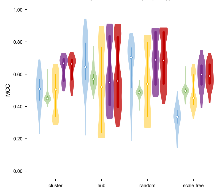
B Synthetic — MCC by topology
