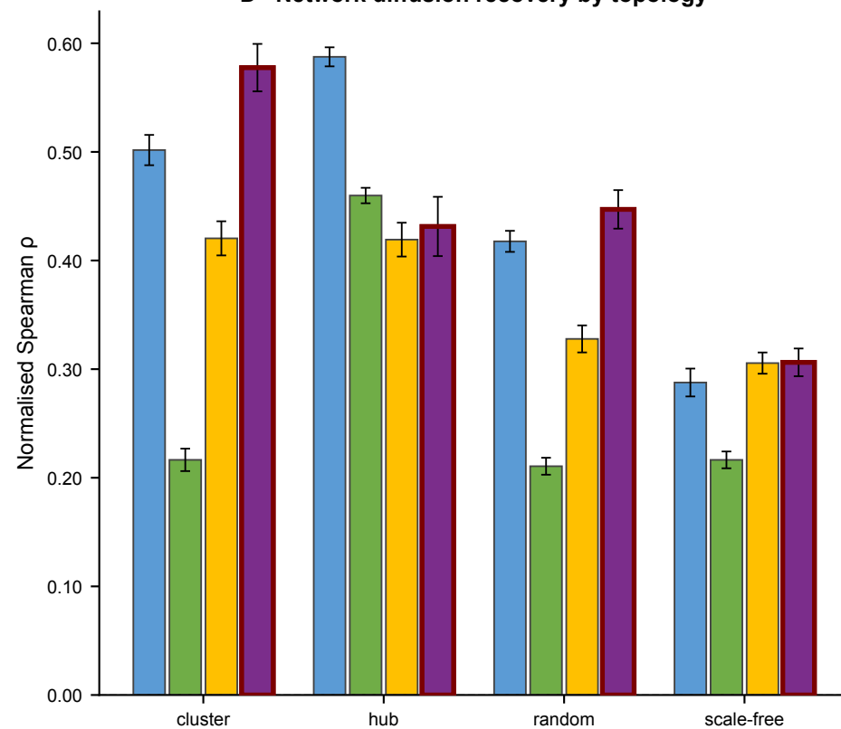
D Network diffusion recovery by topology
