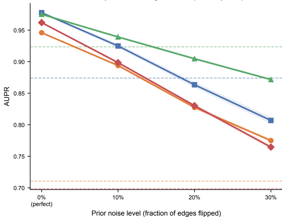
A Oracle prior sensitivity — AUPR (n=513, p=164)
