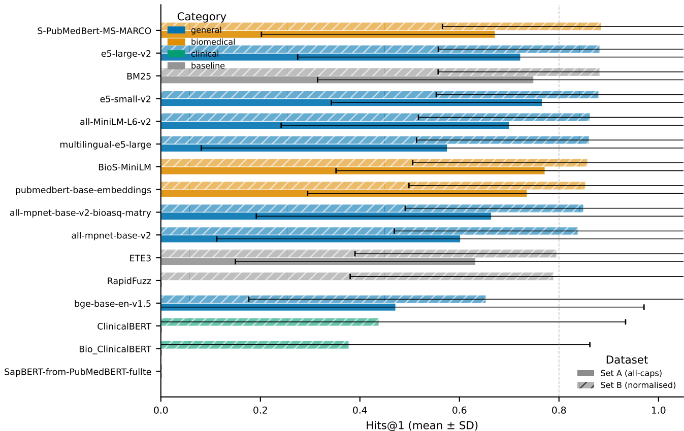
Embedding Model Comparison — MIMIC-IV Ontology Matching
