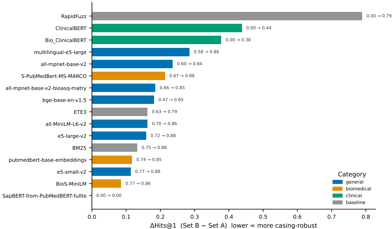
Casing Sensitivity: Performance Drop on All-Caps Clinical Notation
