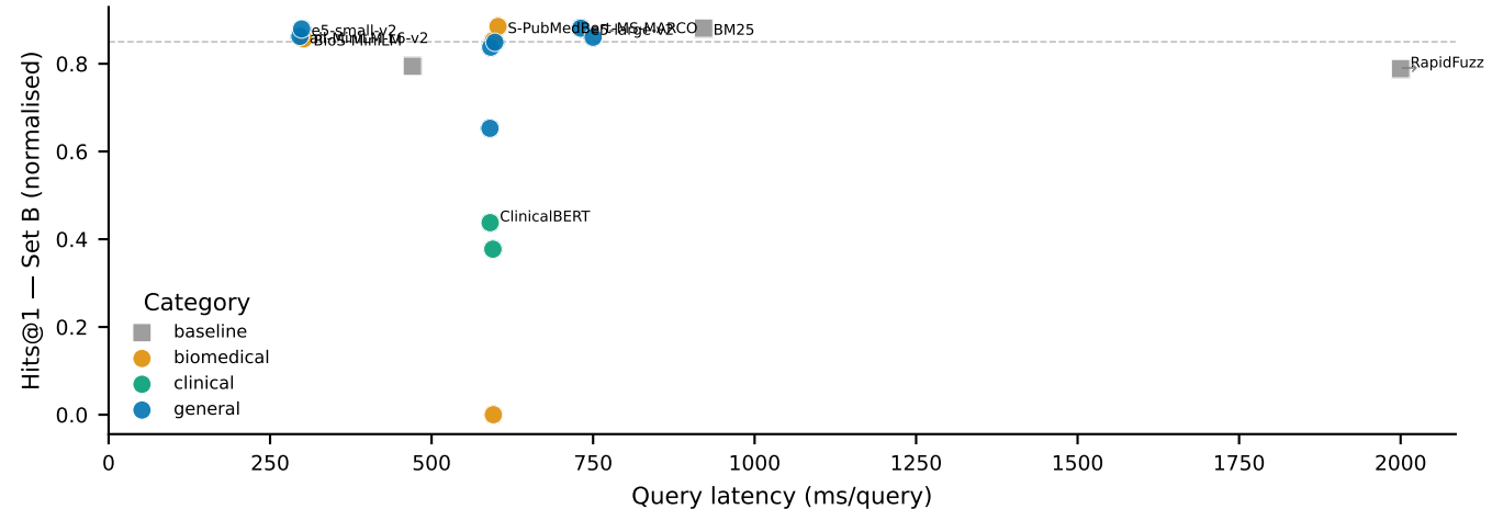
Speed vs. Accuracy Trade-off (Set B)
