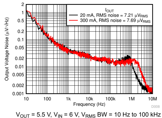
Figure 5-72. Noise vs Frequency and I_{OUT}
