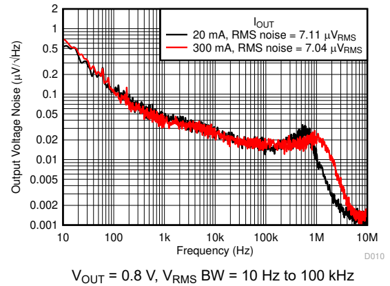
Figure 5-70. Noise vs Frequency and I_{OUT}
