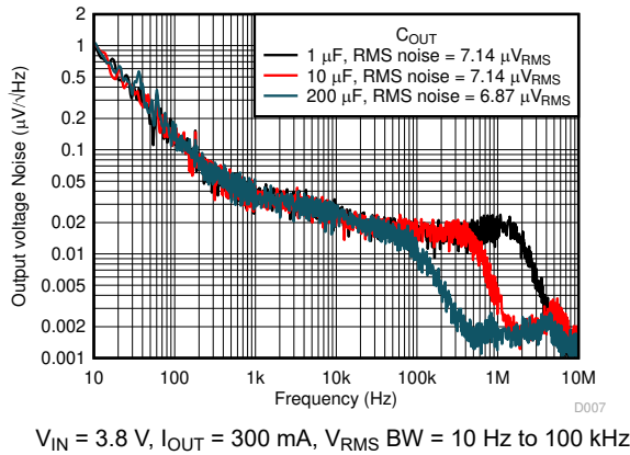
Figure 5-69. Noise vs Frequency and C_{OUT}
