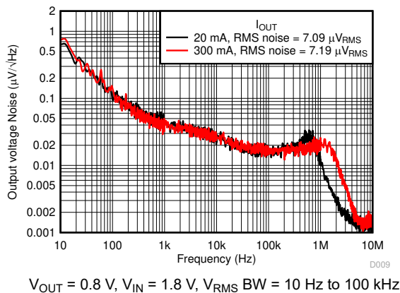
Figure 5-71. Noise vs Frequency and I_{OUT}
