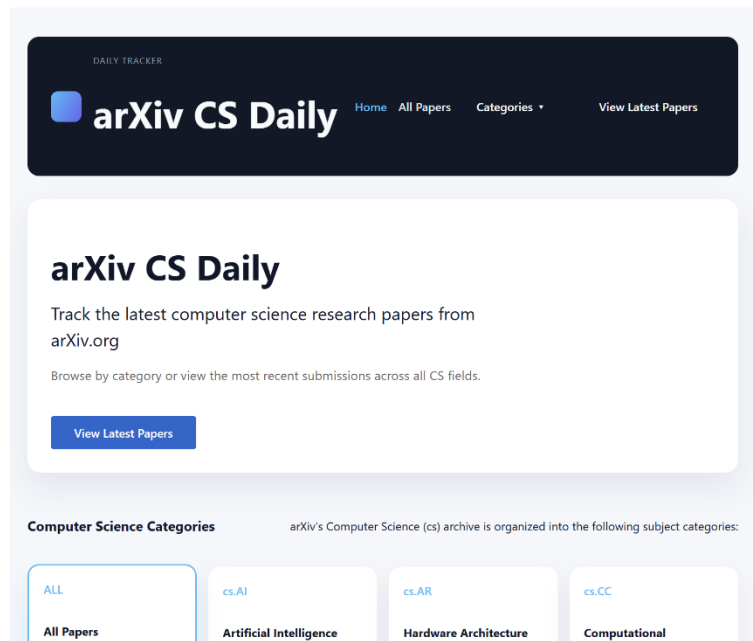
Figure 2 Homepage Overview
