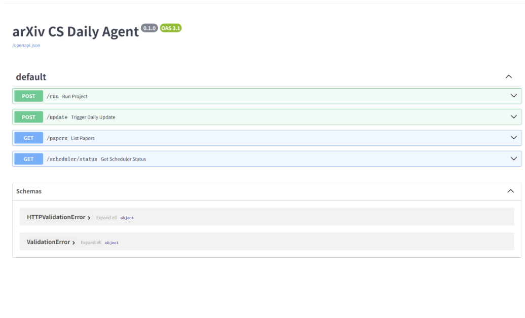
Figure 5 Backend Overview
