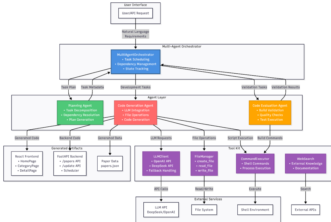
Figure 1 Architecture Overview
