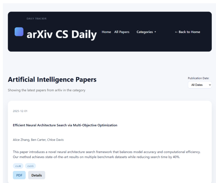
Figure 3 CategoryPage Overview
