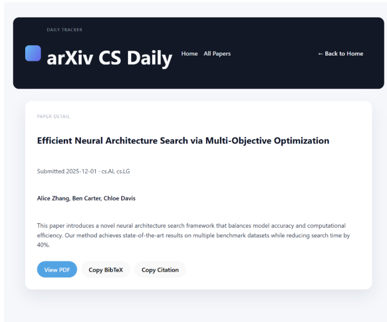
Figure 4 DetailPage Overview
