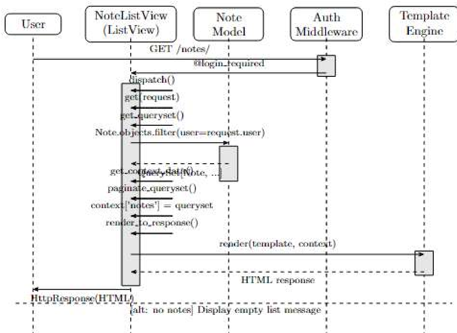
Figure 10: Note List Retrieval Sequence.
