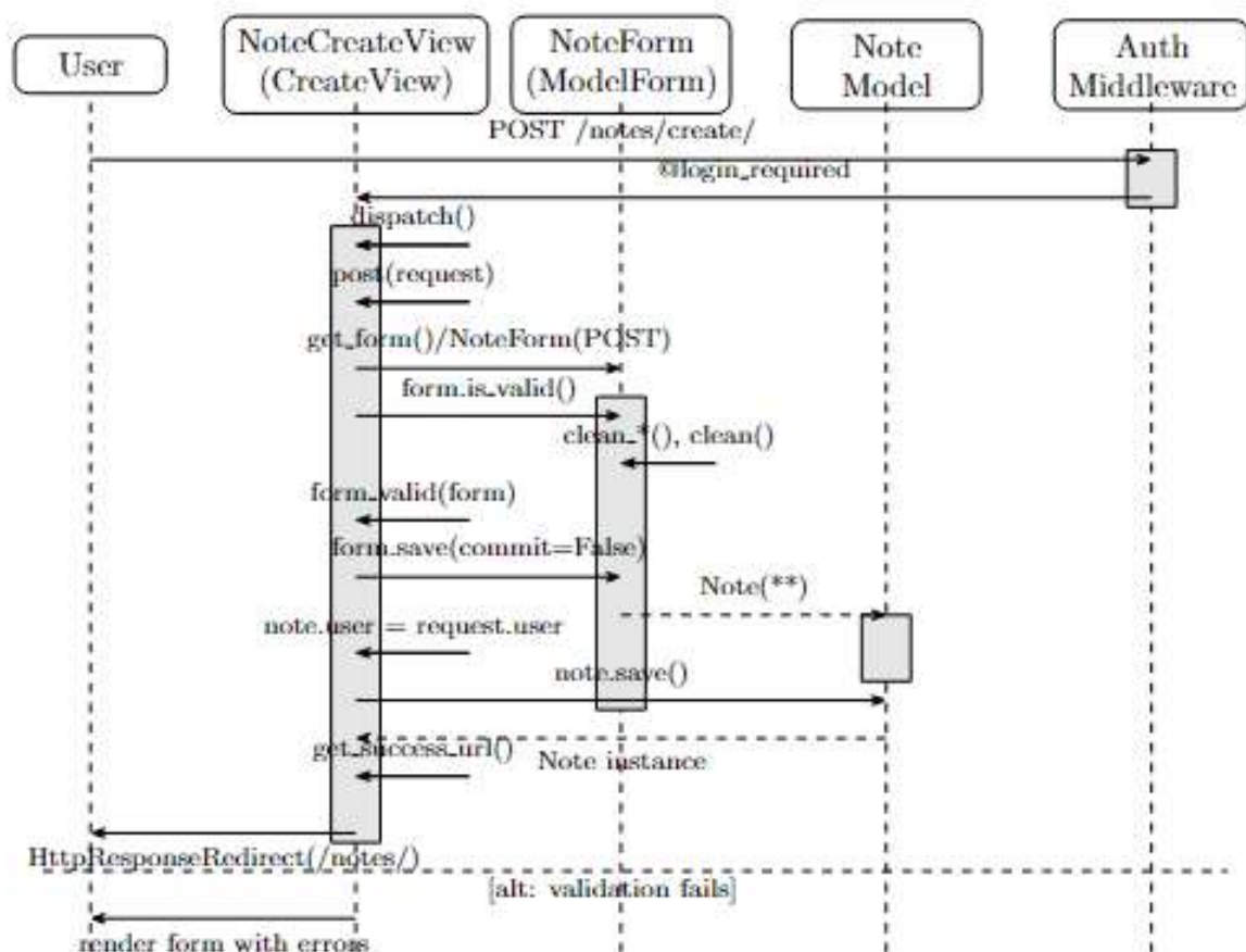
Figure 9: Corrected sequence diagram for creating a note in Django Notejam (POST → authentication → form validation → user association → save → redirect).
