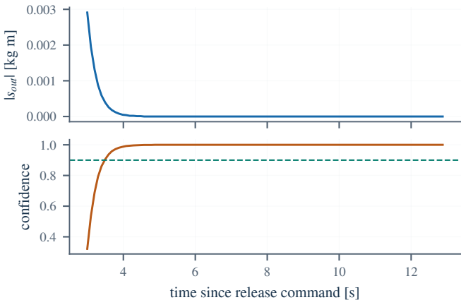
Published release transient (same flight)
