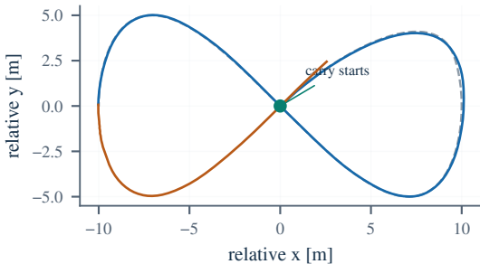
(a) Measured horizontal path
