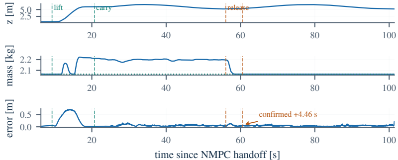
(b) Recorded grasp–carry–release flight
