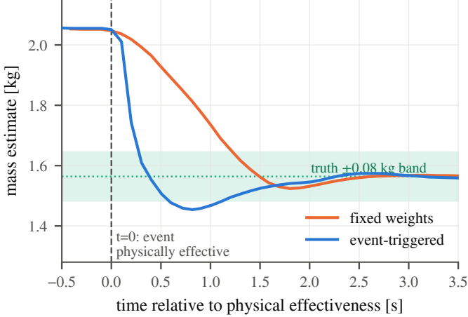
Fig. 2. Mass-estimate timeline (wrench step, \delta m = -0.5 kg). The event-triggered estimate reaches the truth band far earlier than fixed weights, at the cost of a transient overshoot below the band before settling—the speed/overshoot trade-off reported honestly.
