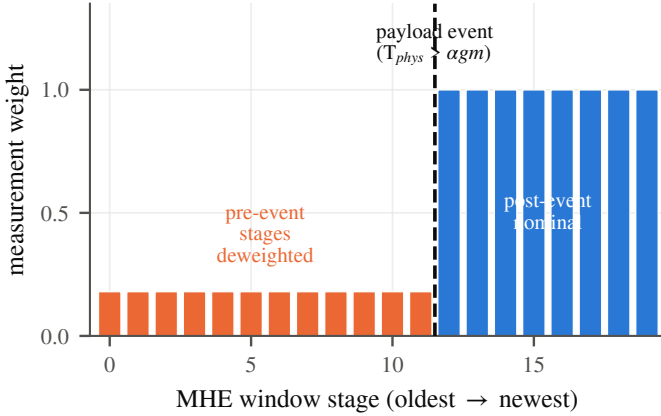
Fig. 2. Sliding-window deweighting. On a payload event (thrust residual crossing \alpha_{gm} ), the pre-event window stages are deweighted so stale cross-discontinuity measurements no longer pull the mass estimate.
