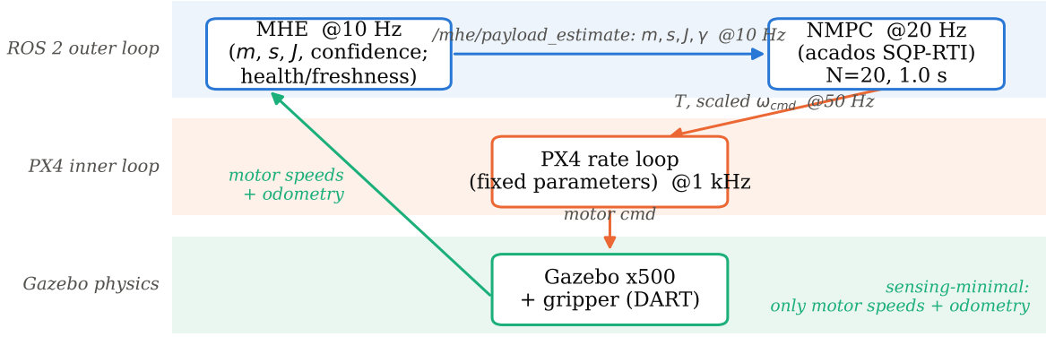
Fig. 1. System architecture and information flow. The full pipeline consumes only motor speeds and odometry; one atomic, health-gated m/s/J frame drives both the NMPC model and continuous rate-command scheduling. No attach/drop notification enters this path.
