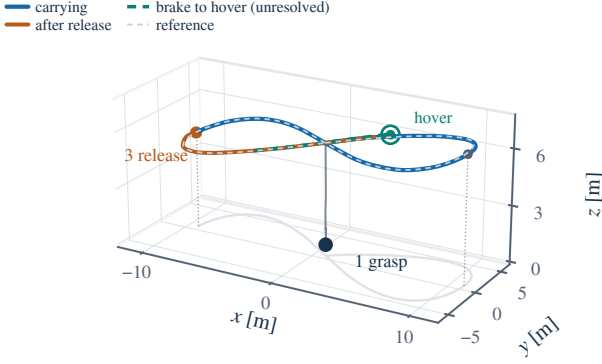
Fig. 2. Measured mission trajectory (simulator ground truth), two 0.15 kg/2 m/s flights of the same batch: grasp (1), lift, then carry along the figure-eight with \pm 0.8 m vertical undulation (blue) against the nominal reference (pale dashed). After the release command (3) one flight clears the moment vote in maneuver and keeps tracking (orange); the other declares UNRESOLVED at its 12 s timeout and brakes to a hover (teal), confirming at 16.40 s. The two paths agree to within 0.12 m (median) before the timeout; loaded tracking RMS is 0.053 m, and 0.060 m after release.
