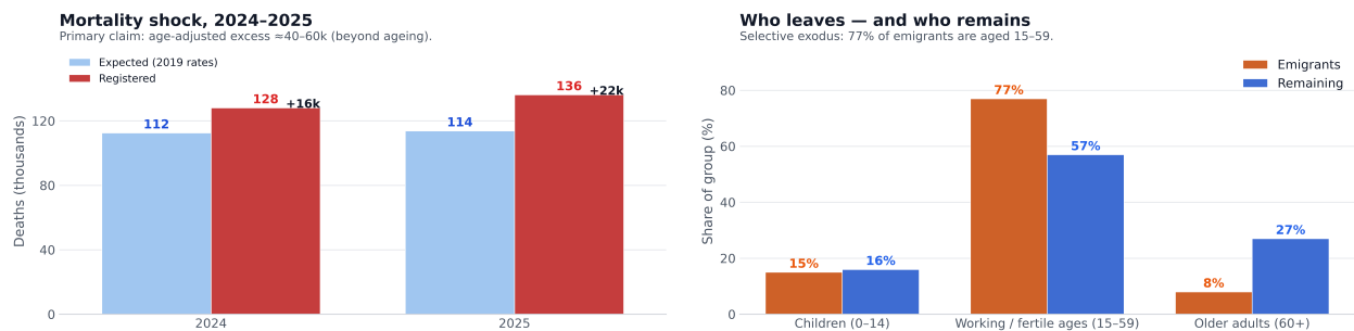
(a) Registered deaths versus an aged 2019-schedule expectation. Primary claim: age-adjusted excess \approx 40\text{--}60 thousand in 2024–2025. Crude registered excess \sim 153,000 over 2020–2025 is a separate quantity. (b) Age composition of emigrants versus remaining residents.
