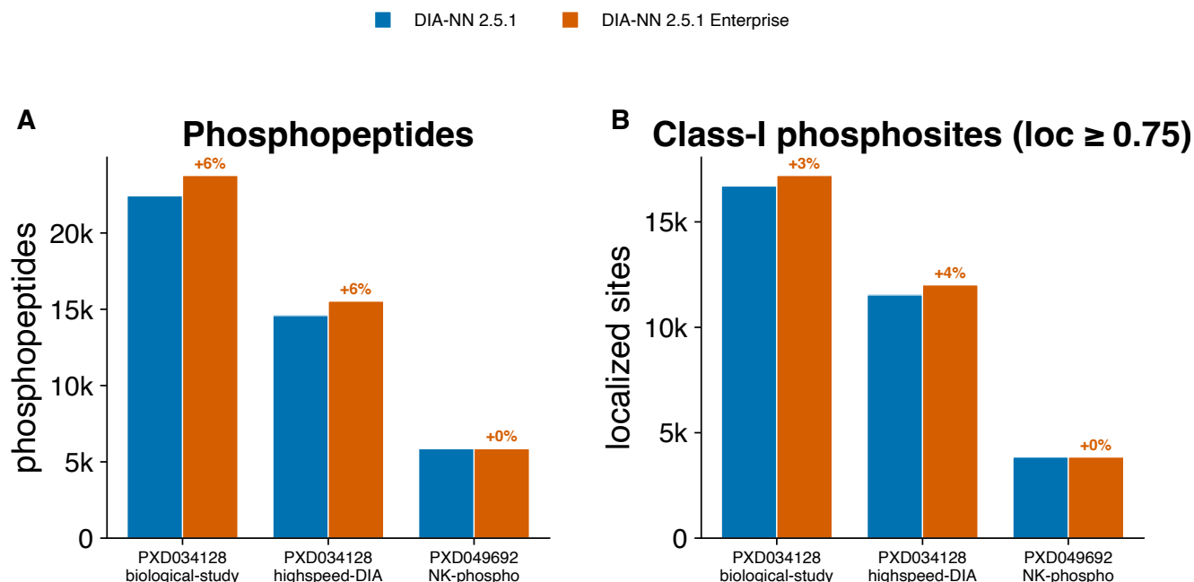
Figure S12: Phosphoproteomics reanalysis by quantmsdiann (DIA-NN, max. two variable modifications per peptide, 1% FDR). (a) Phosphopeptides (distinct phospho-bearing modified precursors) and (b) class-I phosphosites (localization probability \geq 0.75 , unique by protein and residue) for the phospho-enriched cohorts under standard DIA-NN 2.5.1 versus 2.5.1-enterprise: PXD034128 (HeLa EGF, biological-study and high-speed acquisitions) and PXD049692 (NK-cell Fe-NTA diaPASEF). The enterprise build adds a few percent of identifications across both metrics. Phosphoproteomic identification numbers are not compared across search engines (false-localisation rates differ markedly at equal nominal confidence), so only quantmsdiann DIA-NN 2.5.1 counts are shown. The non-enriched PXD034623 (Galectin-1 DIA) is reanalysed for completeness but omitted here, as its \sim 280 phosphopeptides are not comparable to the enriched cohorts.
