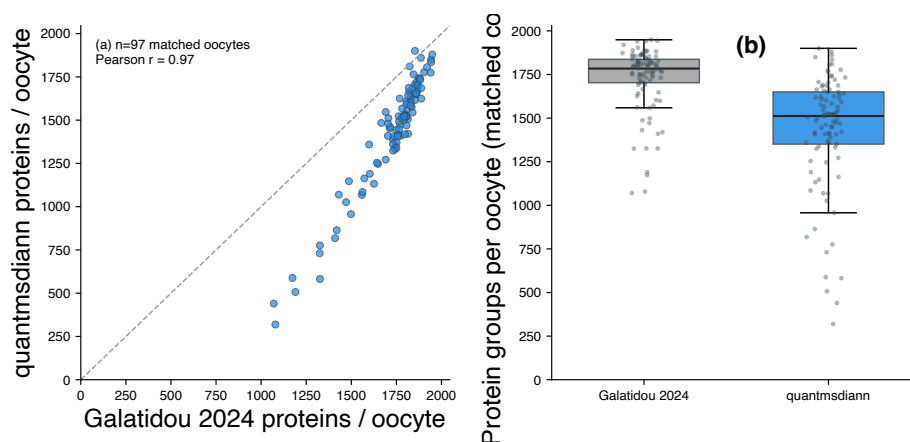
Figure S9: MSV000093870 (Galatidou 2024, single-cell oocyte plexDIA): quantmsdiann reproduces the deposited single-cell depth. For plexDIA, protein-group identification counts are not comparable across DIA-NN versions (the channel-level PG.Q.Value used here is not defined in the DIA-NN 1.8.1 output of the original analysis), so we assess reproducibility rather than an identification gain. (a) Protein groups per single cell, shown for distributional context only (Galatidou n = 97 post-QC 10 oocytes at their reported depth; quantmsdiann n = 107 channel-confident cells at the channel-level PG.Q.Value gate): the two distributions are of comparable magnitude (per-cell median 1.784 versus 1.484) and this panel is not an identification-count comparison. (b) QC-matched
