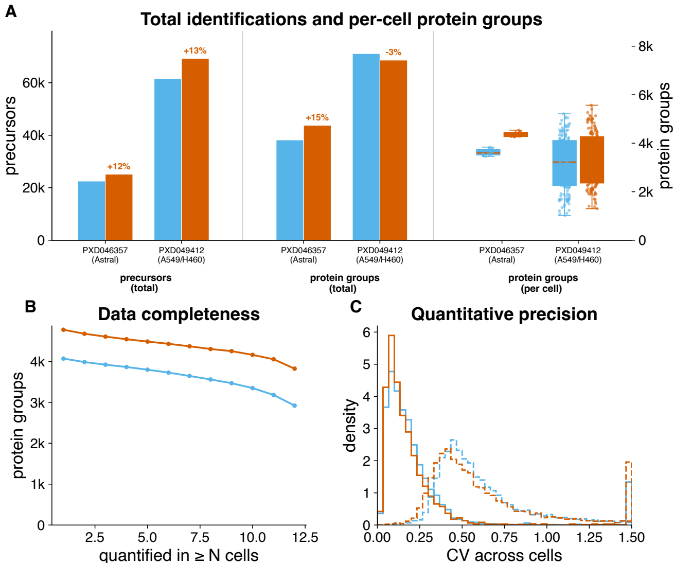
Figure 4: Single-cell DIA reanalysis by quantmsdiann, comparing DIA-NN 1.8.1 with the current 2.5.1-enterprise build on identical raw data. Two label-free Orbitrap Astral single-cell cohorts are shown: HeLa (PXD046357) and a larger A549/H460 cohort of 146 single cells (PXD049412; the 20x/40x A549 library runs are excluded from per-cell counts). (a) Total identifications and per-cell depth, per build, for both cohorts: total precursors (left axis) and total protein groups together with the per-cell protein-group distribution (box and jittered points; right axis); the per-build percentage change is annotated. The A549/H460 cohort reaches comparable per-cell depth on many more cells, but its total protein-group count is already saturated (so the version effect is concentrated in precursor depth). (b) Data-completeness curve for the HeLa Astral flagship: protein groups quantified in at least N cells, the match-between-runs signature, where the right endpoint is the complete-profile count. (c) Distribution of per-protein coefficient of variation across cells for both cohorts (HeLa solid, A549/H460 dashed), summarising quantitative precision; the larger A549/H460 cohort shows the expected higher cell-to-cell variability.
