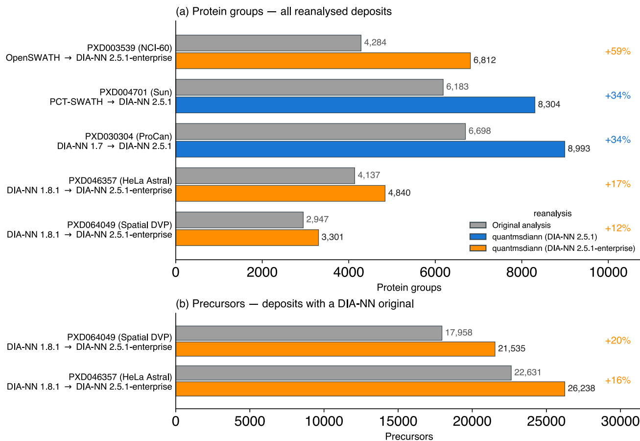
Figure 4: Reanalysis with current DIA-NN identifies more than the originally deposited analyses. Each public DIA deposit is shown as the originally deposited or published count (grey) versus the quantmsdiann reanalysis (coloured by the DIA-NN version used: 2.5.1 or 2.5.1-enterprise), sorted by gain. (a) Protein groups for the five reanalysed deposits, spanning single-cell (HeLa Astral, PXD046357), bulk cell-line (NCI-60, PXD003539; ProCan, PXD030304; Sun, PXD004701) and spatial Deep Visual Proteomics (PXD064049). The multiplexed plexDIA cohort (MSV000093870) is not shown: plexDIA protein-group counts are not comparable across DIA-NN versions. (b) Precursors, restricted to the two deposits with a DIA-NN-based original precursor count (HeLa Astral and spatial DVP); the OpenSWATH/PCT-SWATH originals provide no comparable precursor count. The quantmsdiann side is counted from the per-precursor report (parquet) for all cohorts; the original side is the deposit's count matrix or published headline, except for the spatial cohort, where both the deposited DIA-NN 1.8.1 and quantmsdiann counts are taken from their per-precursor reports under the same global rule (Supplementary Note 3), and over the identical 12 quantified runs on both sides (the deposited DIA-NN log loads additional library/QC runs that are not in the deposited quantification matrix). The five-cohort pan-cohort integration (per-tissue coverage) is in Supplementary Fig. S7.
