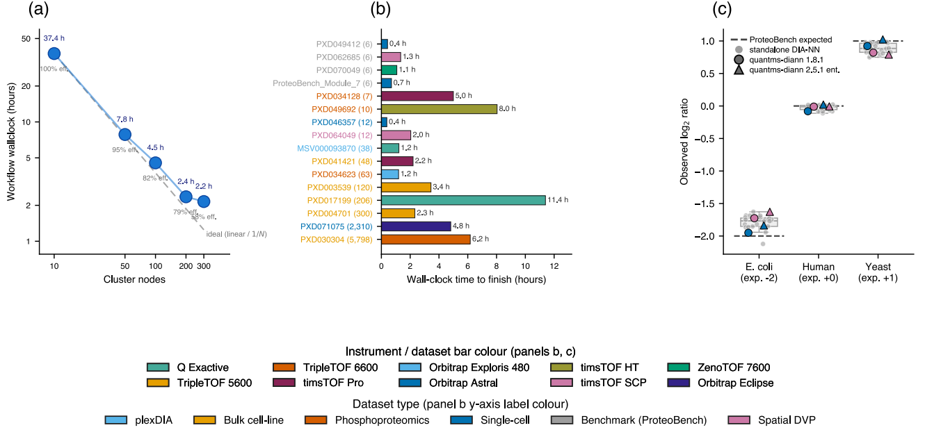
Figure 2: Runtime scaling and ProteoBench quantification accuracy. (a) Workflow wall-clock versus number of cluster nodes (Nextflow executor.queueSize ) on the PXD071075 single-cell cohort (log-log; one run per point). The dashed grey line is ideal 1/N scaling anchored at 10 nodes; parallel efficiency is printed under each dot. The curve bends above ideal beyond \sim 100 nodes (efficiency 100% \rightarrow 58%), reflecting fixed serial cohort-level steps and shared-cluster contention on this EMBL-EBI allocation. (b) Wall-clock per reanalysis, one bar per dataset, ordered by cohort size and coloured by instrument family; the dataset-type metadata is shown by the colour of each cohort's y-axis label (descriptive only: bar height reflects cohort size and parallelisation, not sample type per se). (c) ProteoBench accuracy per HYE species: observed log 2 fold-change against the expected ratio (dashed) for the two DIA modules with predicted-from-FASTA DIA-NN submissions (Orbitrap Astral, Module 7; timsTOF diaPASEF, Module 5, PXD062685). Standalone community runs (all versions) form the grey strip and box; quantmsdiann points are coloured by instrument and shaped by DIA-NN version (circle, 1.8.1; triangle, 2.5.1-enterprise), tracking the community distribution, i.e. distributed orchestration does not change quantification accuracy.
