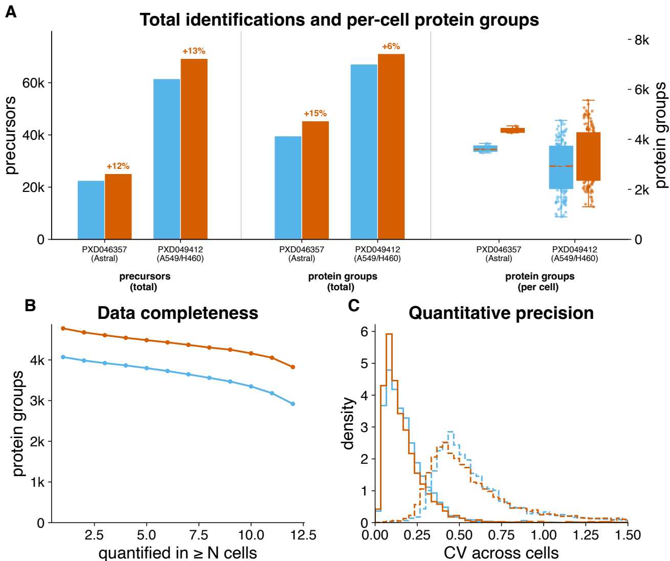
Figure 3: Single-cell DIA reanalysis by quantmsdiann, comparing DIA-NN 1.8.1 with the current 2.5.1-enterprise build on identical raw data. Two label-free Orbitrap Astral single-cell cohorts are shown: HeLa (PXD046357) and a larger A549/H460 cohort of 146 single cells (PXD049412; the 20x/40x A549 library runs are excluded from per-cell counts). (a) Total identifications and per-cell depth, per build, for both cohorts: total precursors (left axis) and total protein groups together with the per-cell protein-group distribution (box and jittered points; right axis); the per-build percentage change is annotated. The A549/H460 cohort reaches comparable per-cell depth on many more cells, but its total protein-group count is already saturated (so the version effect is concentrated in precursor depth). (b) Data-completeness curve for the HeLa Astral flagship: protein groups quantified in at least N cells, the match-between-runs signature, where the right endpoint is the complete-profile count. (c) Distribution of per-protein coefficient of variation across cells for both cohorts (HeLa solid, A549/H460 dashed), summarising quantitative precision (axis truncated at CV = 1.5 ); the larger A549/H460 cohort shows the expected higher cell-to-cell variability.
