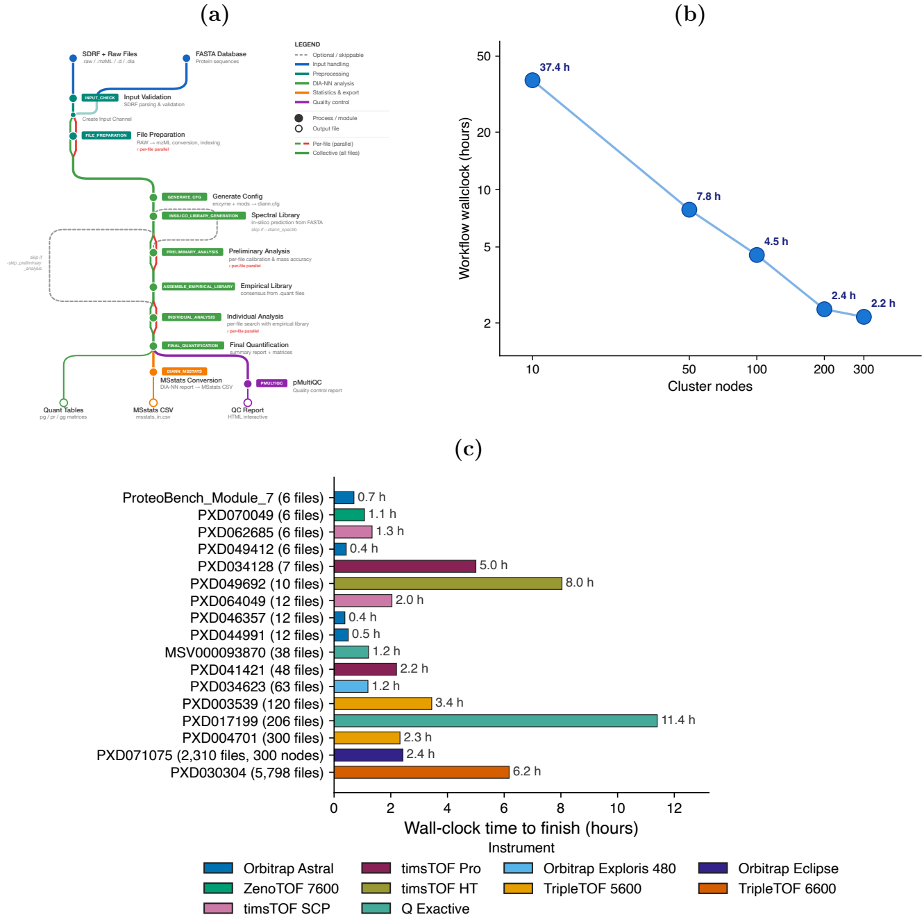
Figure 1: quantmsdiann pipeline architecture and runtime scaling. (a) Subway diagram of the quantmsdiann workflow: mandatory modules as filled circles, optional/skippable modules as open circles. Per-file parallel stages (red; file preparation, preliminary calibration, individual search) run as one task per raw file, whereas collective stages (green; in-silico library generation, empirical library assembly, final quantification, MSstats conversion, and pmultiqc reporting) run once over the full cohort. (b) Workflow wall-clock time versus the number of cluster nodes (Nextflow executor.queueSize ) on the PXD071075 single-cell cohort. (c) Wall-clock time to finish each reanalysis, one bar per dataset, ordered by cohort size (number of MS data files) and coloured by instrument family. In both (b) and (c) the reported time excludes the in-silico spectral-library prediction step ( INSILICO_LIBRARY_GENERATION ), a one-time, cohort-independent cost that can be predicted once and reused, so the bars reflect the per-file quantification work. Time-to-finish stays within a few hours across two orders of magnitude in file count because per-file stages are parallelised across the cluster; the deeper variable-modification search of the phosphoproteomics cohorts (e.g. PXD049692) is the main residual driver of wall-clock once library prediction is set aside.
