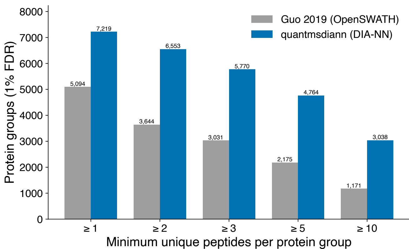
Figure S5: PXD003539: distribution of peptides per protein group. quantmsdiann (DIA-NN, blue) versus Guo 2019 OpenSWATH (grey) on the same NCI-60 raw data.
