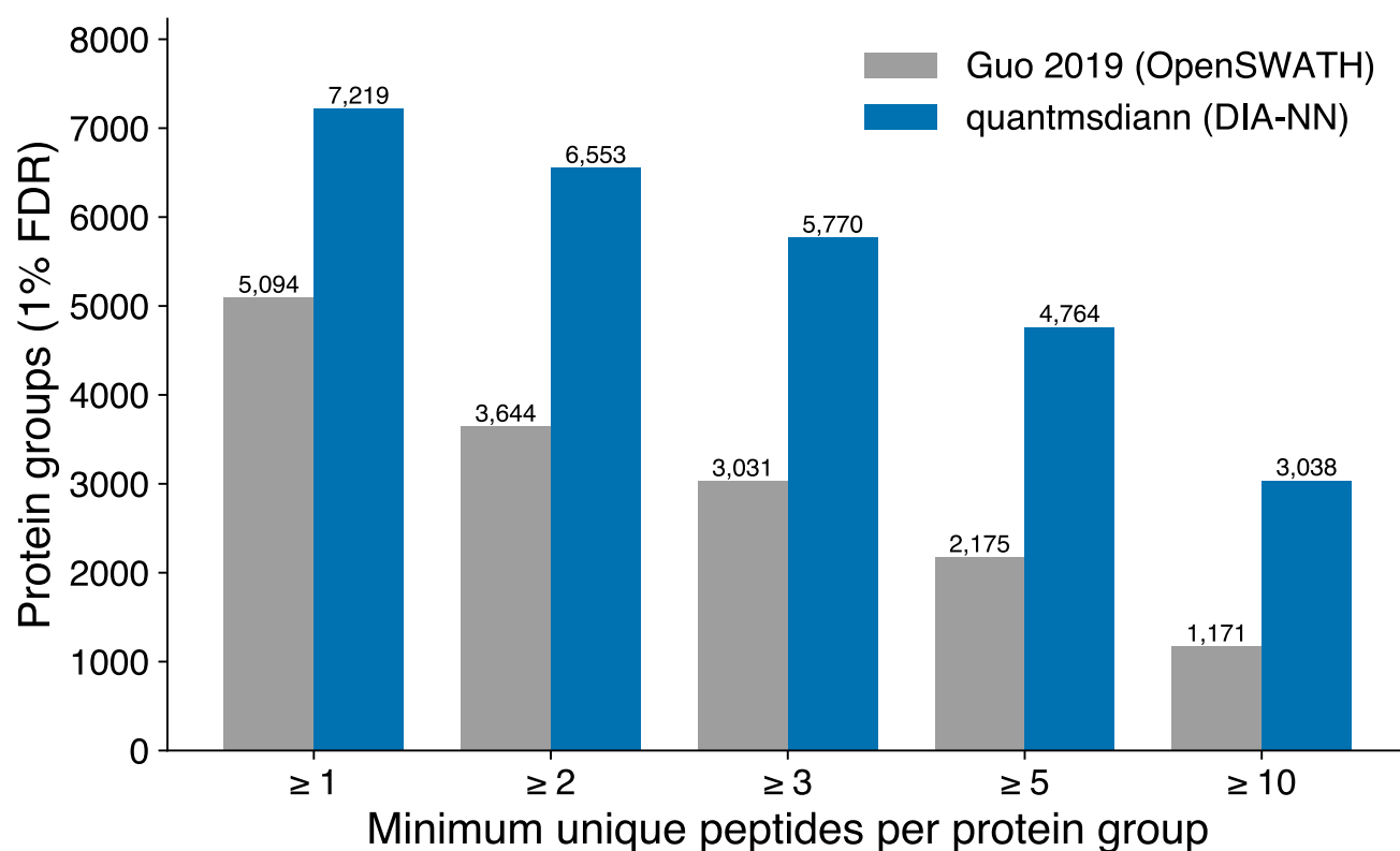
Figure S3: PXD003539: distribution of peptides per protein group. quantmsdiann (DIA-NN, blue) versus Guo 2019 OpenSWATH (grey) on the same NCI-60 raw data.
