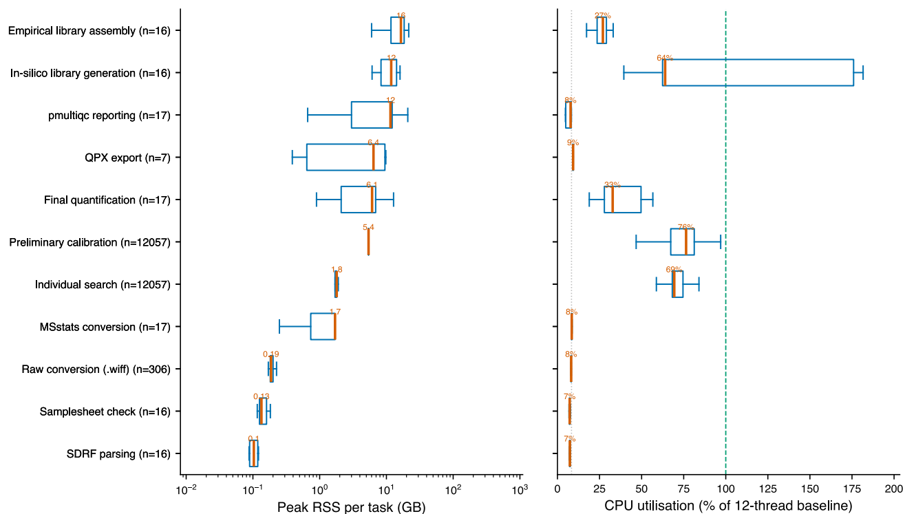
Figure S2: Peak memory and CPU envelope per Nextflow process. Per-task peak resident-set-size memory (left panel) and CPU utilisation (right panel) per quantmsdiann process across the ProteoBench benchmark cohorts and the PXD071075 cluster-node sweep. Box plots show the median (vermillion) and interquartile range; the per-step task count is given in each y-axis label and the median is printed above each box. CPU utilisation is expressed as a percentage of quantmsdiann 's 12-thread DIA-NN allocation, so a step that parallelises beyond its 12 allotted threads exceeds the 100% baseline (green dashed line); the in-silico library-generation step does so, while single-threaded glue steps sit near 1/12 \approx 8\% (grey dotted line). The collective FINAL_QUANTIFICATION stage dominates memory use on large cohorts; per-file stages remain well within the commodity 8–16 GB per-task envelope typical of HPC partitions.
