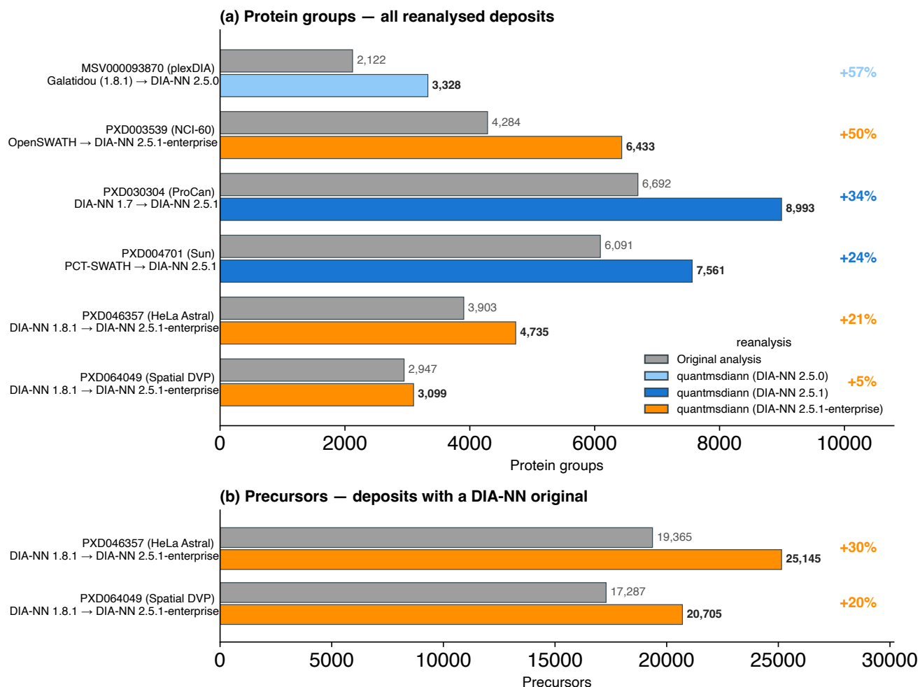
Figure 3: Reanalysis with current DIA-NN recovers more than the originally deposited analyses. Each public DIA deposit is shown as the originally deposited or published count (grey) versus the quantmsdiann reanalysis (coloured by the DIA-NN version used: 2.5.0, 2.5.1, or 2.5.1-enterprise), sorted by gain. (a) Protein groups for all six reanalysed deposits, spanning single-cell (HeLa Astral, PXD046357; plexDIA, MSV000093870), bulk cell-line (NCI-60, PXD003539; ProCan, PXD030304; Sun, PXD004701) and spatial Deep Visual Proteomics (PXD064049). (b) Precursors, restricted to the two deposits with a DIA-NN-based original precursor count (HeLa Astral and spatial DVP); the OpenSWATH/PCT-SWATH originals, and plexDIA (protein-level report only), provide no comparable precursor count. The quantmsdiann side is counted from the precursor report (parquet) and the original side from the deposit's matrix or published headline (Supplementary Note 3). The five-cohort pan-cohort integration (per-tissue coverage) is in Supplementary Fig. S13.
