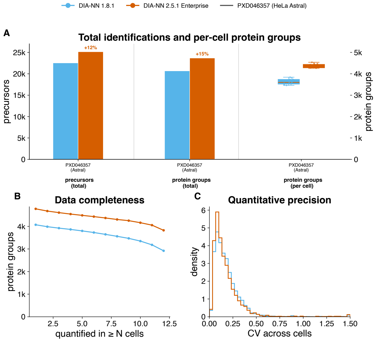
Figure 4: Single-cell DIA reanalysis by quantmsdiann, comparing DIA-NN 1.8.1 with the current 2.5.1-enterprise build on identical raw data. The label-free Orbitrap Astral single-cell HeLa cohort (PXD046357) is shown. (a) Total identifications and per-cell depth, per build: total precursors (left axis) and total protein groups together with the per-cell protein-group distribution (box and jittered points; right axis), the newer build lifting both the totals and per-cell depth; the per-build percentage change is annotated. (b) Data-completeness curve: protein groups quantified in at least N cells, the match-between-runs signature, where the right endpoint is the complete-profile count. (c) Distribution of per-protein coefficient of variation across cells, summarising quantitative precision.
