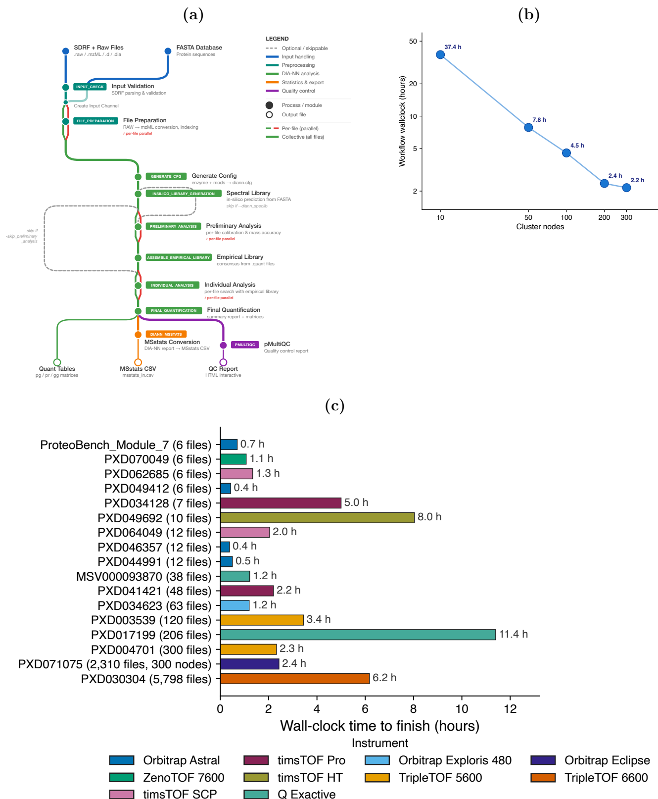
Figure 1: quantmsdiann pipeline architecture and runtime scaling. (a) Subway diagram of the quantmsdiann workflow: mandatory modules as filled circles, optional/skippable modules as open circles. Per-file parallel stages (red; file preparation, preliminary calibration, individual search) run as one task per raw file, whereas collective stages (green; in-silico library generation, empirical library assembly, final quantification, MSstats conversion, and pmultiqc reporting) run once over the full cohort. (b) Workflow wall-clock time versus the number of cluster nodes (Nextflow executor.queueSize ) on the PXD071075 single-cell cohort. (c) Wall-clock time to finish each reanalysis, one bar per dataset, ordered by cohort size (number of MS data files) and coloured by instrument family. In both (b) and (c) the reported time excludes the in-silico spectral-library prediction step ( INSILICO_LIBRARY_GENERATION ), a one-time, cohort-independent cost that can be predicted once and reused, so the bars reflect the per-file quantification time. Times for individual reanalysis of each dataset were obtained from a single analysis of the dataset on a 300-node cluster.
