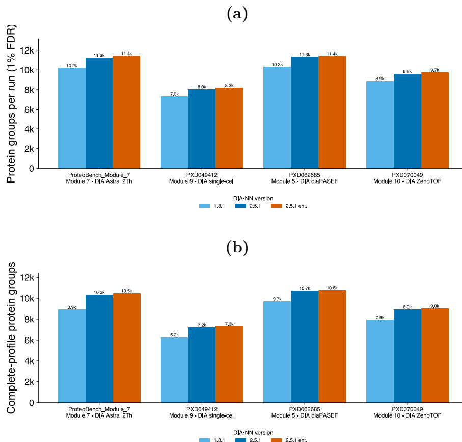
Figure S4: Protein-group depth on ProteoBench across three DIA-NN configurations and four DIA modalities. (a) Protein groups per run (averaged over the six replicates) at a 1% run-specific protein-group FDR, by DIA-NN configuration (1.8.1 and 2.5.1 light to dark blue; 2.5.1-enterprise in amber) from one quantmsdiann invocation. (b) Complete-profile protein groups (quantified in every run). Both metrics rise monotonically from 1.8.1 to 2.5.1 to the enterprise build on every module; the gain is larger for the complete profiles (up to +18% to the enterprise build) than for the per-run average (+10–12%), reflecting improved cross-run consistency in the newer release.
