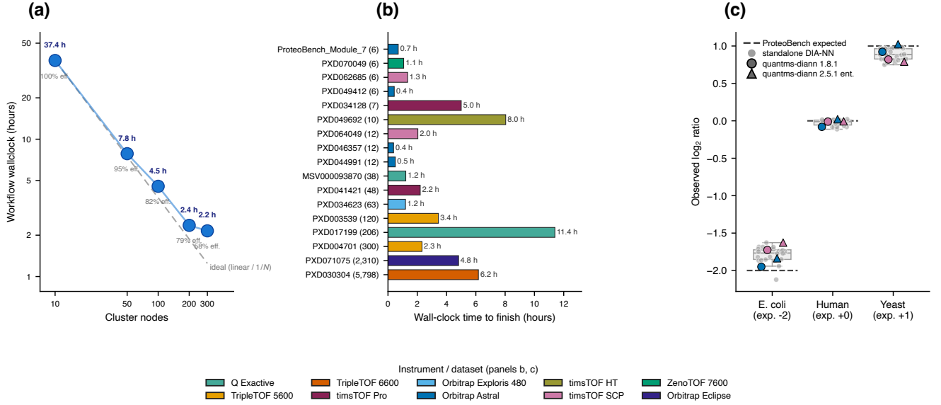
Figure 2: Runtime scaling and ProteoBench quantification accuracy. (a) Workflow wall-clock versus the number of cluster nodes (Nextflow executor.queueSize ) on the PXD071075 single-cell cohort, log-log axes. The dashed grey line is ideal linear ( 1/N ) strong scaling anchored at the 10-node point; parallel efficiency (measured/ideal speed-up) is printed under each dot. The measured curve bends above the ideal beyond \sim 100 nodes (efficiency 100\% \rightarrow 58\% over the sweep), reflecting both the fixed serial cohort-level steps and shared-cluster resource contention at high concurrency on this EMBL-EBI allocation (see text); each point is a single run. (b) Wall-clock time to finish each reanalysis, one bar per dataset, ordered by cohort size and coloured by instrument family; (a) and (b) exclude the one-time in-silico spectral-library prediction, except the PXD003539 bar, whose incomplete execution trace did not allow the library step to be separated, so its bar conservatively includes it (a \sim 0.4 h overstatement relative to the other bars). (c) ProteoBench quantification accuracy per HYE species: observed log 2 fold-change against the ProteoBench-expected ratio (dashed) for the two DIA modules with predicted-from-FASTA DIA-NN community submissions (Orbitrap Astral, Module 7; timsTOF SCP diaPASEF, PXD062685). Standalone DIA-NN community runs (all versions) appear as a grey strip and box; quantmsdiann points are coloured by instrument (shared legend) and shaped by DIA-NN version (circle, 1.8.1; triangle, 2.5.1-enterprise), and track the community distribution across species, i.e. distributed orchestration does not change quantification accuracy. Per-version, per-module identification depth is in Supplementary Note 5 (Fig. S4).
