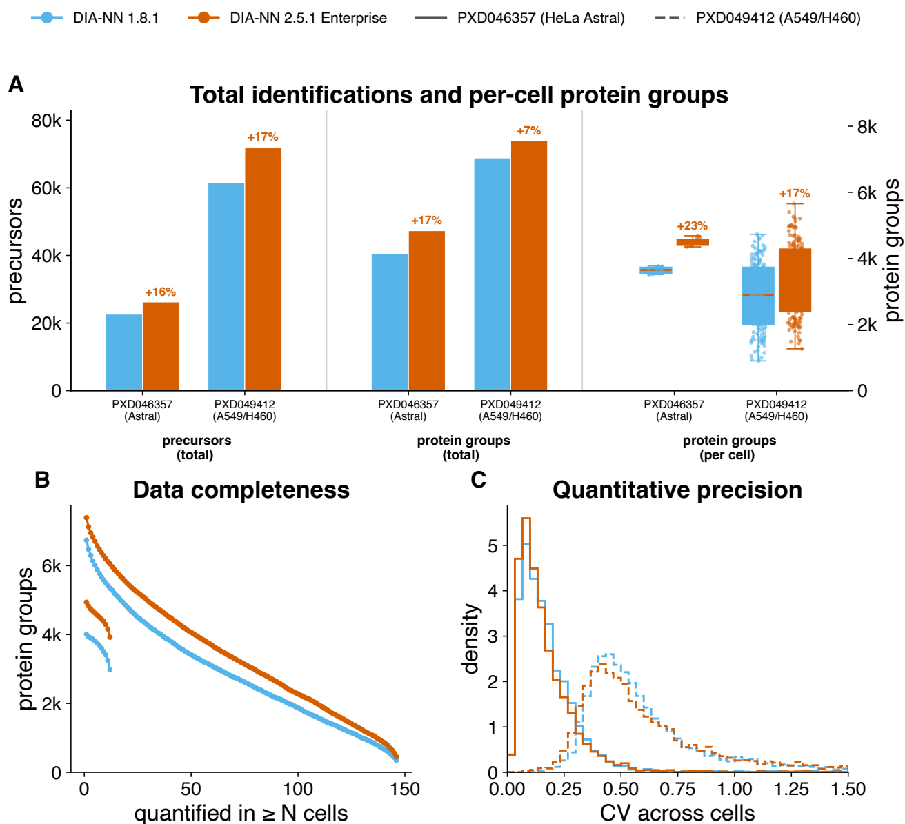
Figure 3: Single-cell DIA reanalysis by quantmsdiann, comparing DIA-NN 1.8.1 with the current 2.5.1-enterprise build on identical raw data. Two label-free Orbitrap Astral single-cell cohorts are shown: HeLa (PXD046357) and a larger A549/H460 cohort of 146 single cells (PXD049412; the 20x/40x A549 library runs are excluded from per-cell counts). (a) Total identifications and per-cell depth, per build, for both cohorts: total precursors (left axis) and total protein groups together with the per-cell protein-group distribution (box and jittered points; right axis); the per-build percentage change is annotated. The A549/H460 cohort reaches comparable per-cell depth on many more cells, but its total protein-group count is already saturated (so the version effect is concentrated in precursor depth). (b) Data-completeness curves for both single-cell cohorts (HeLa Astral, solid; A549/H460, dashed): protein groups quantified in at least N cells, the match-between-runs signature, where the right endpoint is the complete-profile count. (c) Distribution of per-protein coefficient of variation across cells for both cohorts (HeLa solid, A549/H460 dashed), summarising quantitative precision (axis truncated at CV = 1.5 ); the larger A549/H460 cohort shows the expected higher cell-to-cell variability.
