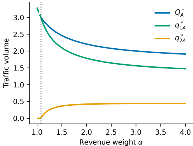
(a) Model A ( \Delta = 7.5 )
