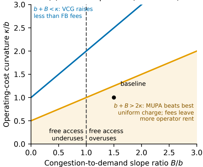
(a) Static comparisons (Models A-B)
