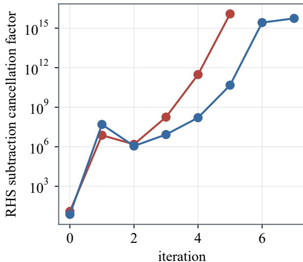
(b) Floating-point resolution diagnostic
