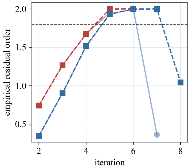
(a) Binary64 and binary128 order
