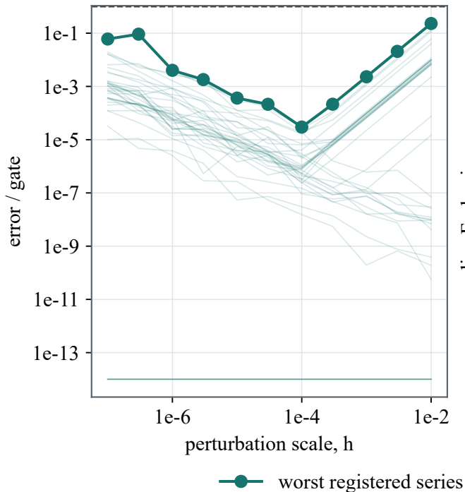
(a) Branchwise KSS directional audit
