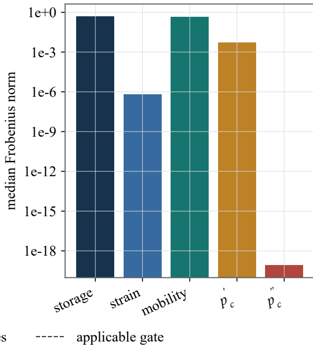
(b) KSS term ledger
