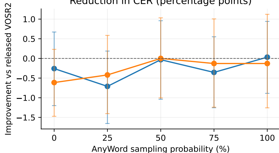
Reduction in CER (percentage points)
