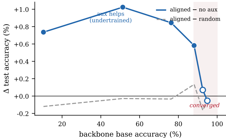
(a) CIFAR-10: the benefit saturates
