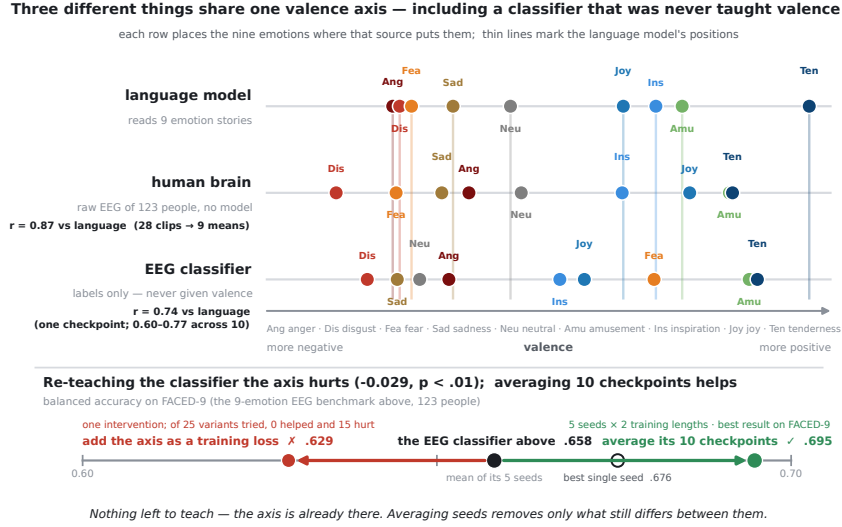
Figure 1: A converged classifier rejects the concept it already learned—in one view. Top: a valence axis ( V -axis) from nine language-model emotion stories orders the nine FACED emotions; the same ordering appears in the cohort human EEG ( r=0.87 over 28 clips) and, without ever being supervised on it, in a converged EEG classifier’s class means ( |r| \in [0.60, 0.77] across ten checkpoints). Thin lines mark the language model’s positions. Bottom: the converged classifier has already absorbed the concept, so adding the V -axis as an auxiliary loss lowers FACED-9 balanced accuracy ( 0.658 \rightarrow 0.629 , \Delta = -0.029 , p < 0.01 ; of 25 variants, 0 help and 15 hurt), whereas averaging its ten checkpoints—which share the axis but differ in their seed-specific residual—sets a new state of the art ( 0.6948 ; best single model 0.6755 ).
