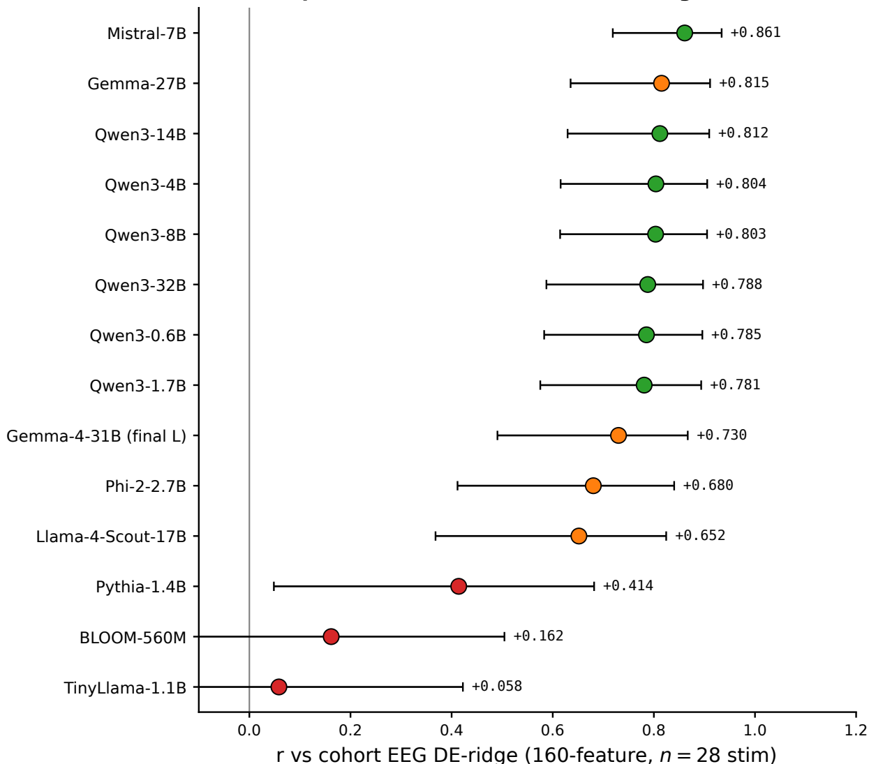
(a) Brain prediction: r vs cohort EEG-DE-Ridge
