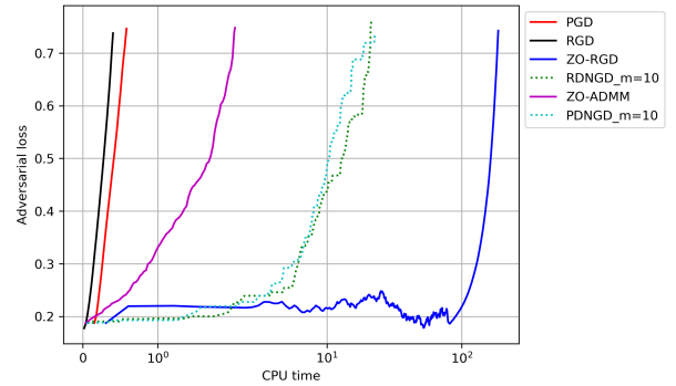
Figure 9: Additional attack result on CIFAR-10 (Example 2).
