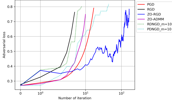
Figure 8: Additional attack result on CIFAR-10 (Example 1).
