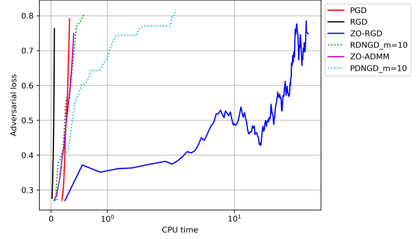
Figure 8: Additional attack result on CIFAR-10 (Example 1).
