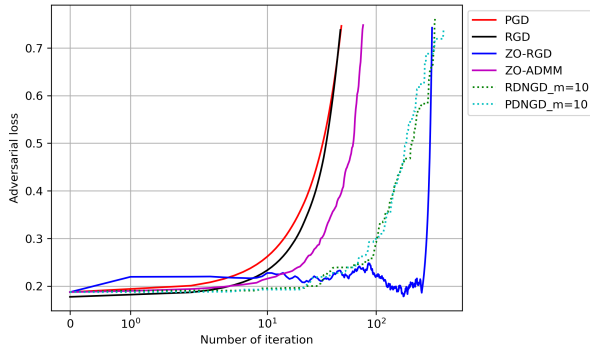
Figure 9: Additional attack result on CIFAR-10 (Example 2).
