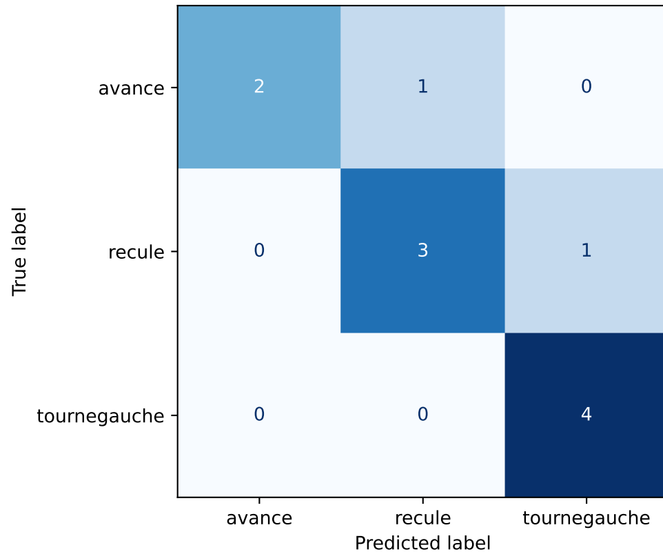
Test — Acc=81.82%
