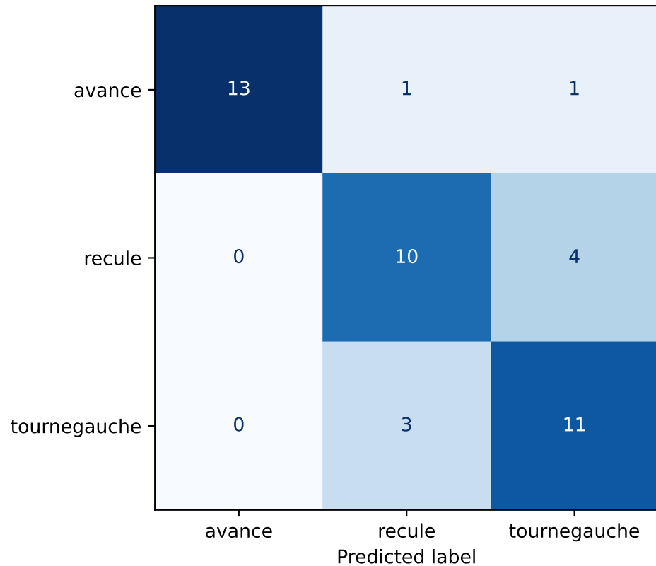
Train (LOO) — Acc=79.07%
