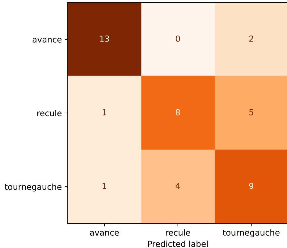
Train (LOO) — Acc=69.77%
