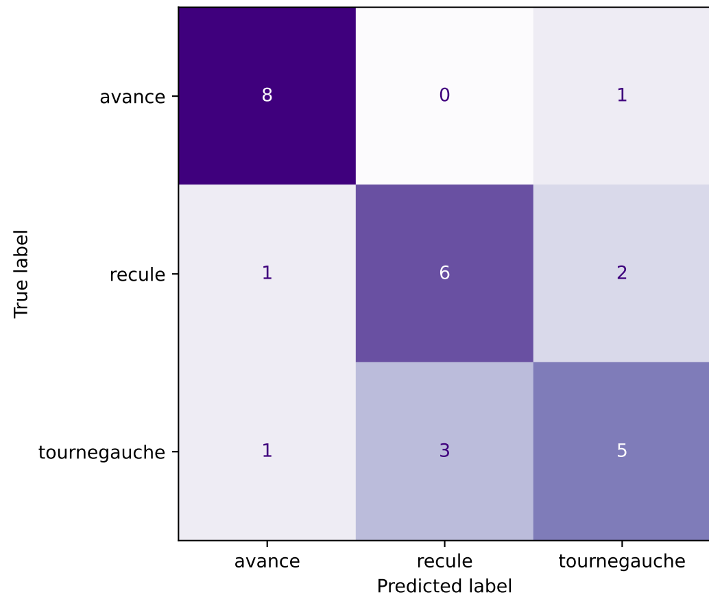
CNN 1D — Acc=70.37%
