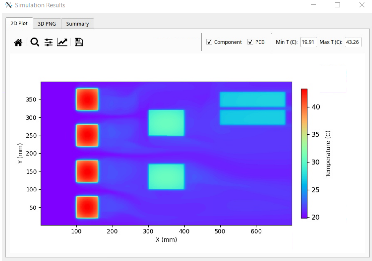
Figure 12: PowerSynth-MOSTCOOL Solution window.
