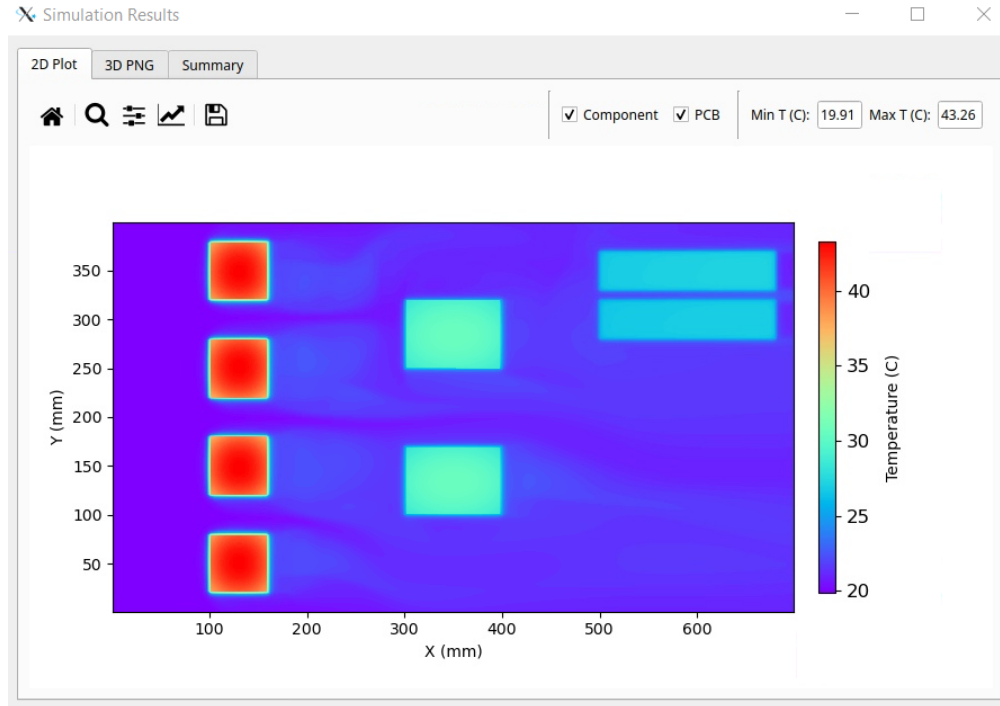
Figure 5: PowerSynth-MOSTCOOL solution window: 2D Plot tab
