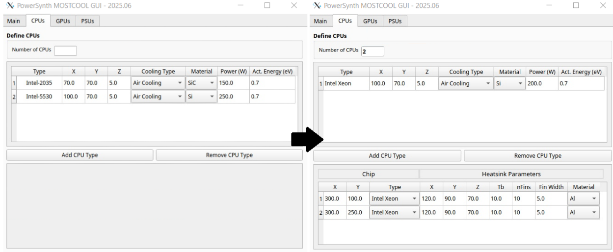
Figure 2: PowerSynth-MOSTCOOL CPUs tab: Initial and Final setting up parameters
