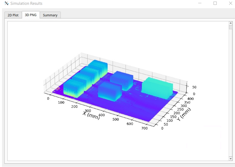
Figure 6: PowerSynth-MOSTCOOL solution window: 3D PNG tab
