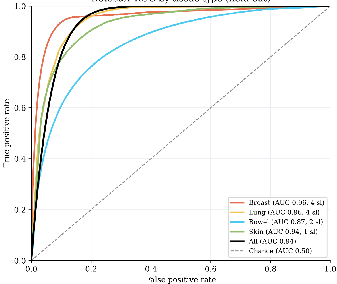
Detector ROC by tissue type (held-out)
