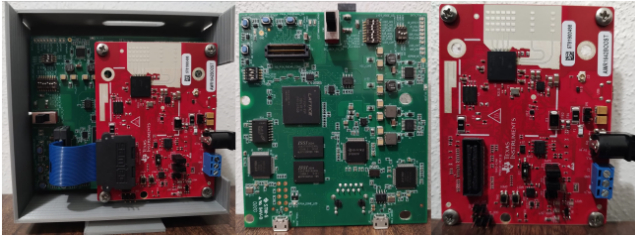
Figure 1: AWR1642 EVM - DCA1000- AWR1642 and DCA1000 in the designed radar holder (from right to left)
