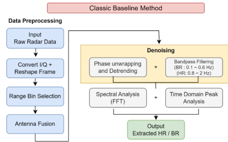
Figure 3: Classical baseline approach architecture
