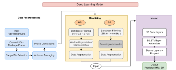
Figure 5: deep learning approach architecture
