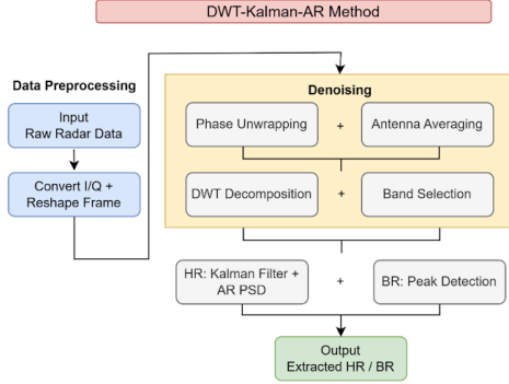
Figure 4: DWT-Kalman-AR approach architecture
